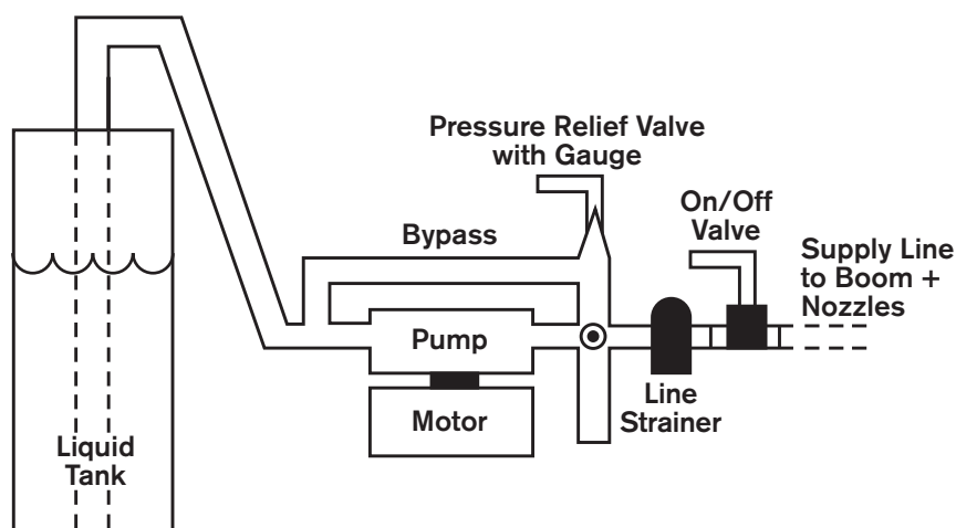
Pump System
